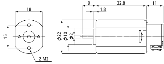
DN22 S+Encoder 62P/R
